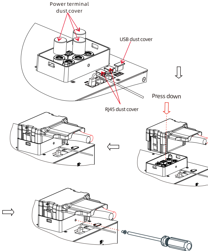
Fig 4.8: Power connection
