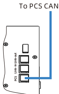
Fig 4.7: Single cluster communication wiring
