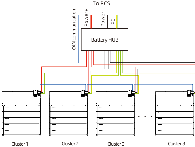
Fig 4.9: Block diagram of multi-cluster system
