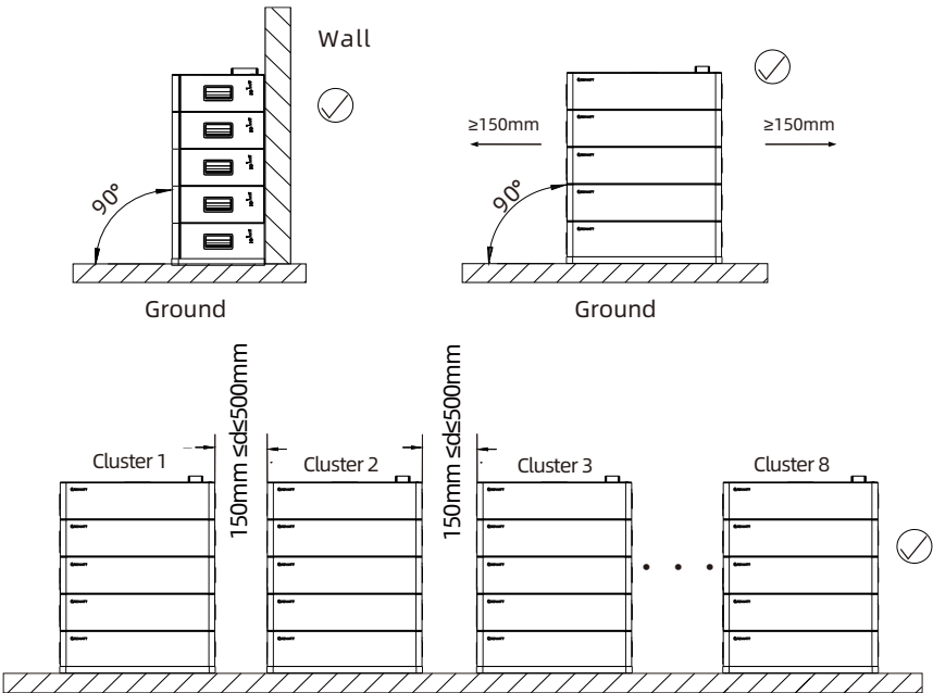
Ground(2 ~ 8 clusters installation)
