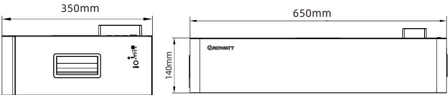
Fig 1.1: Battery size diagram
